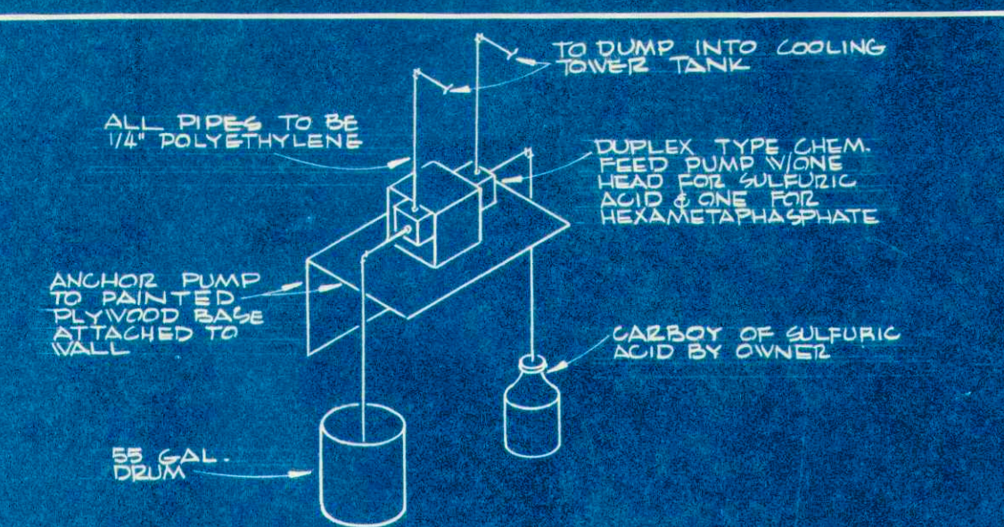
CHEMICAL FEED PUMP ISOMETRIC NO SCALE
