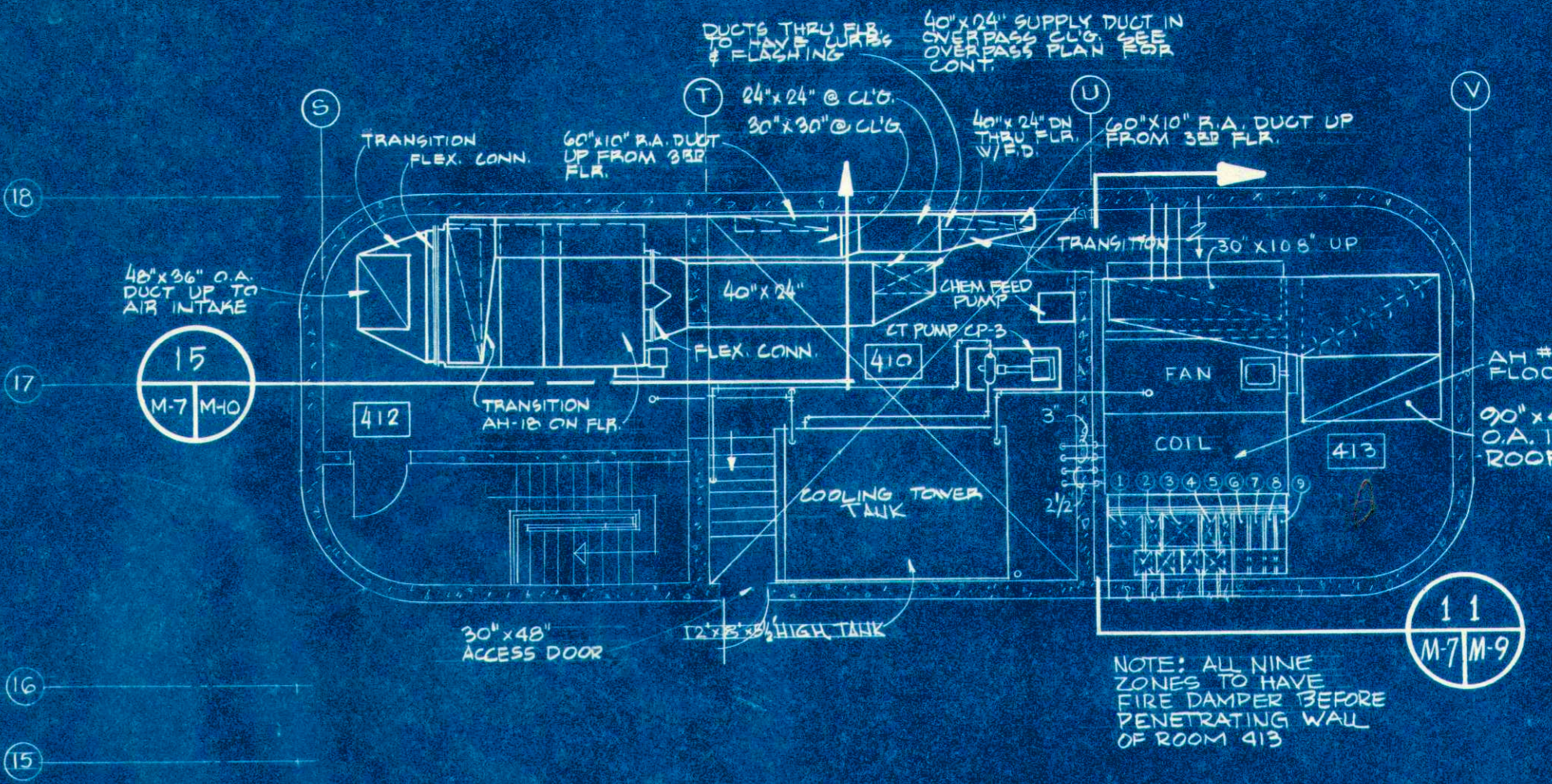
FOURTH FLOOR TOWER AREA 1/8" = 1'-0"
