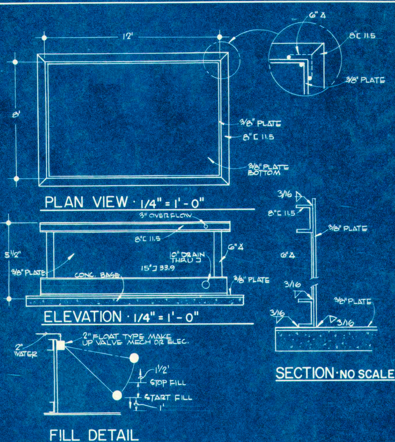
COOLING TOWER TANK DETAIL SCALE AS NOTED
