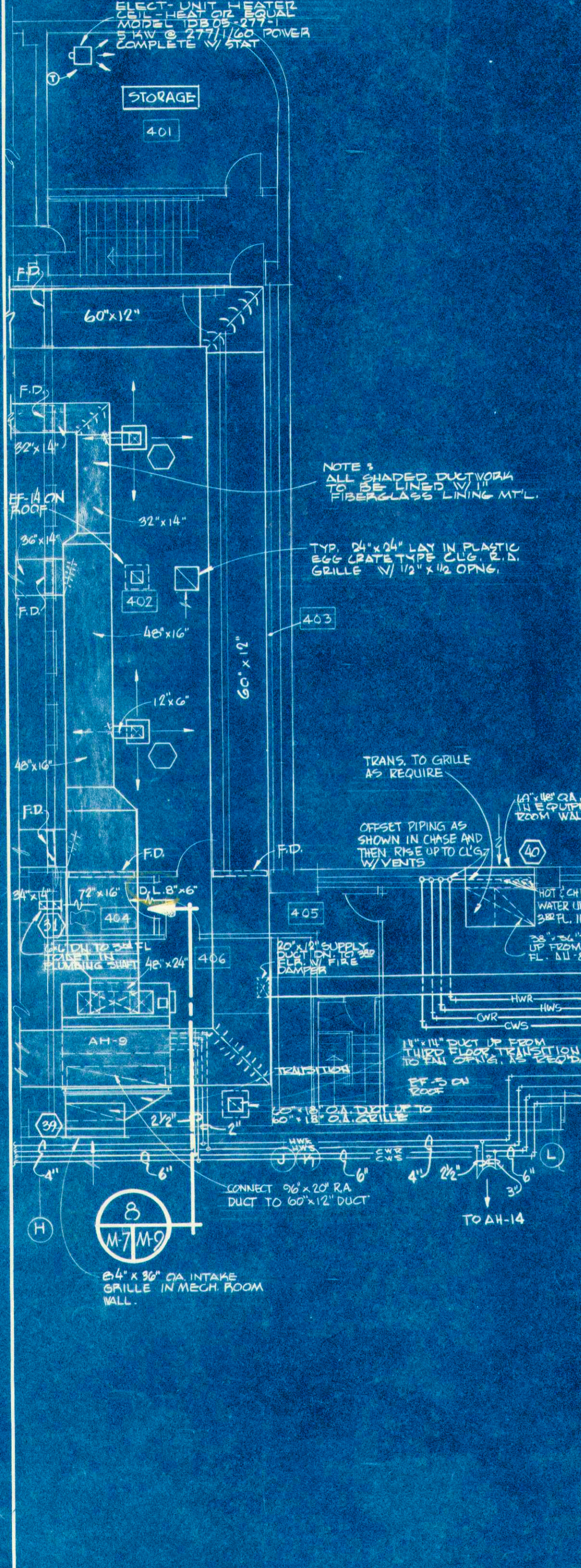
FOURTH FLOOR PLAN-EQUIPMENT ROOM 1/8" = 1'-0"
