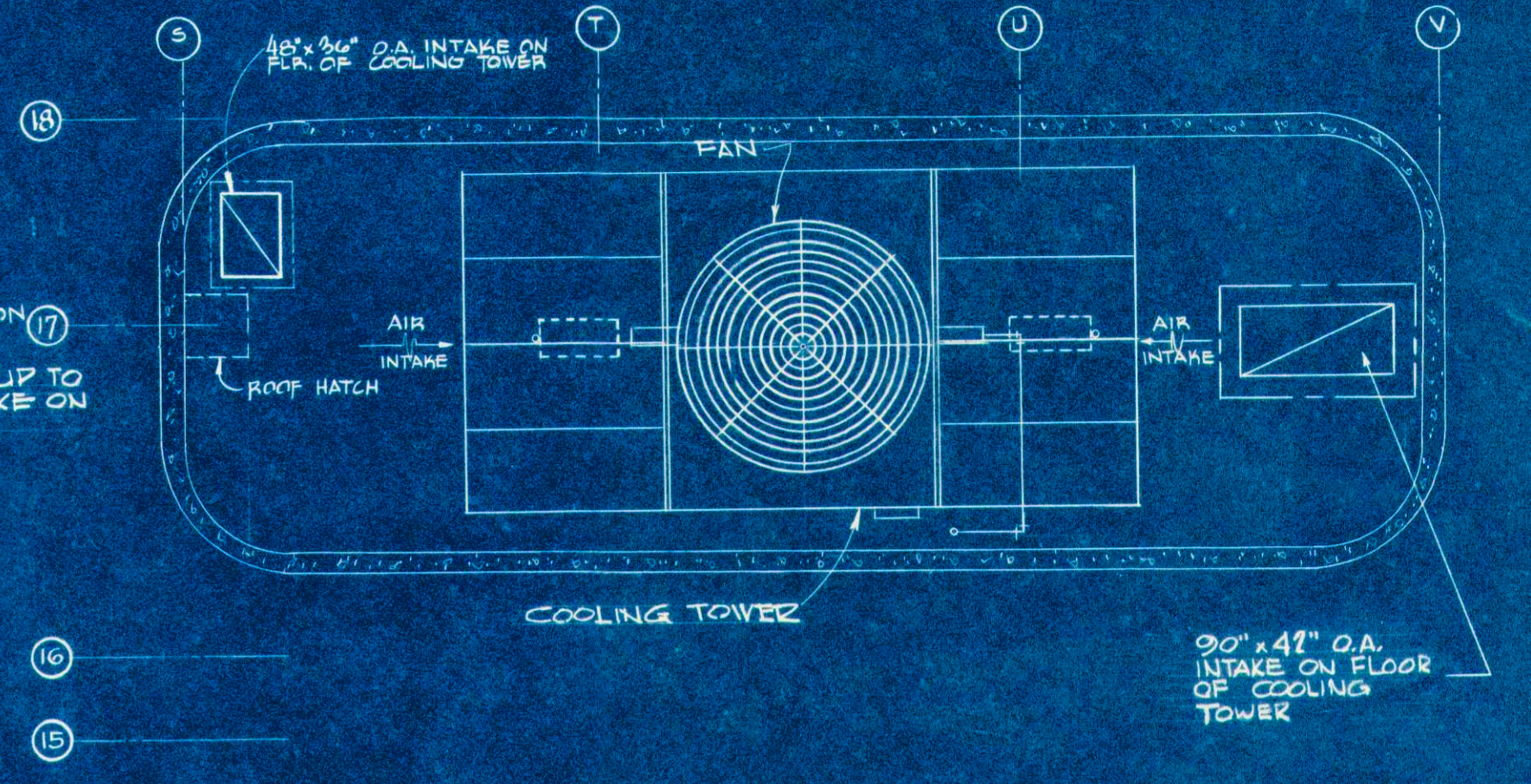
COOLING TOWER FLOOR PLAN 1/8" = 1'-0"
